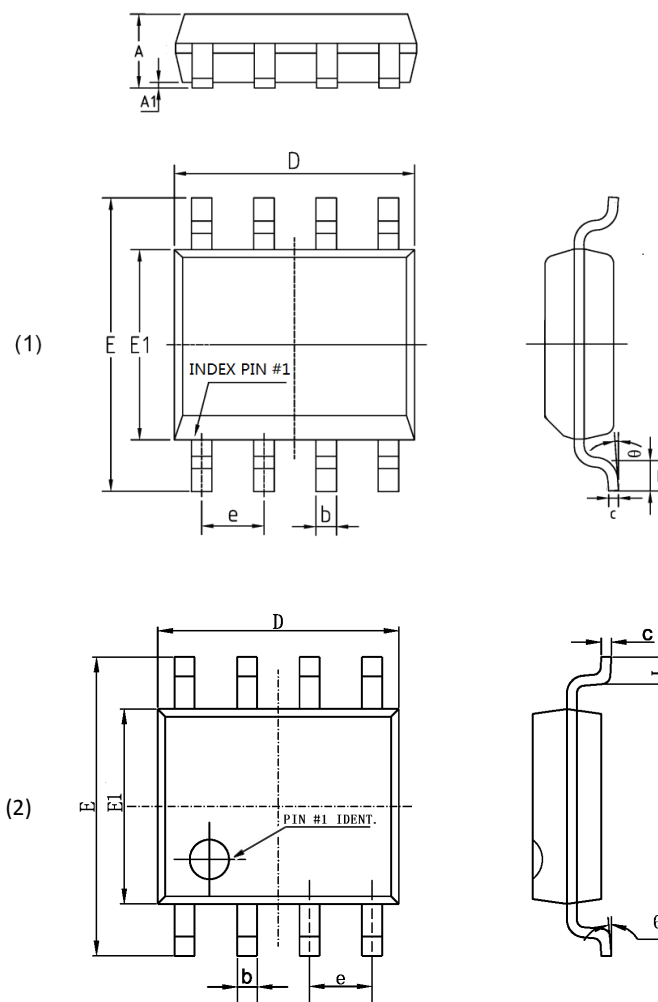
SOP8 (150mil)
