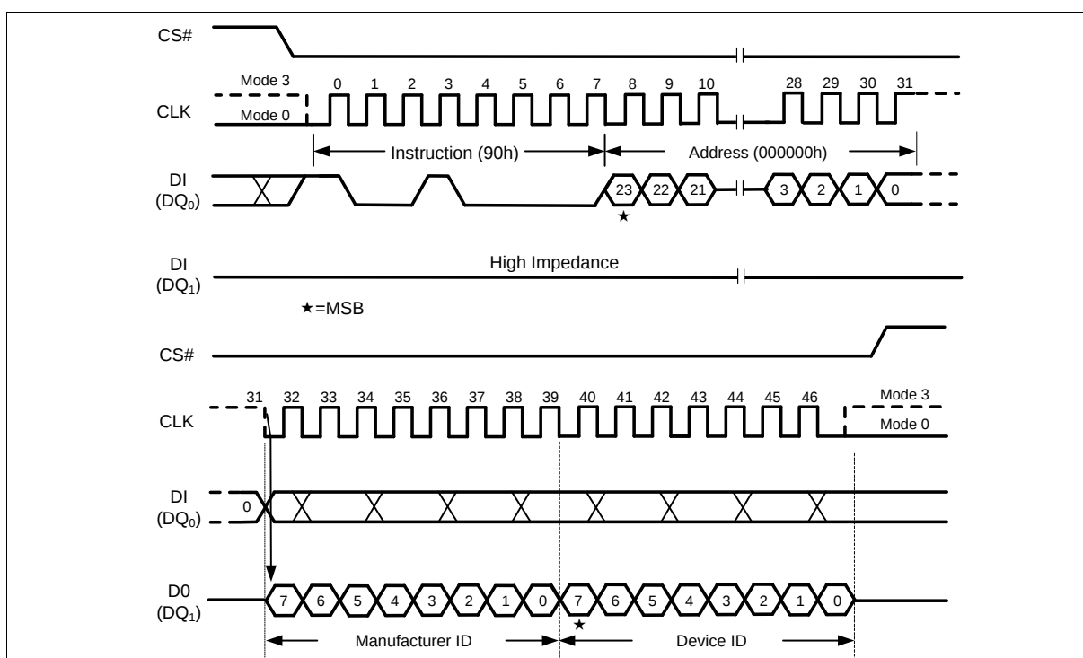
Figure 48 Read Manufacturer / Device ID Instruction (SPI Mode)
