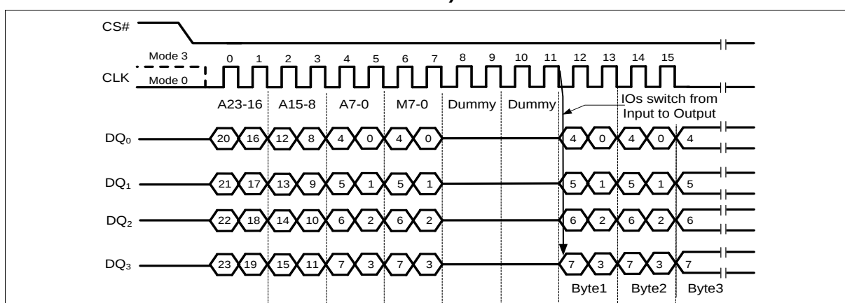
Figure 25 Fast Read Quad I/O Instruction (Previous instruction set M5-4 = 10, SPI Mode)
